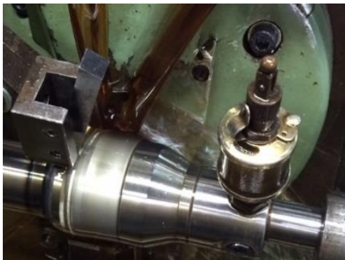
Gear hobbing
